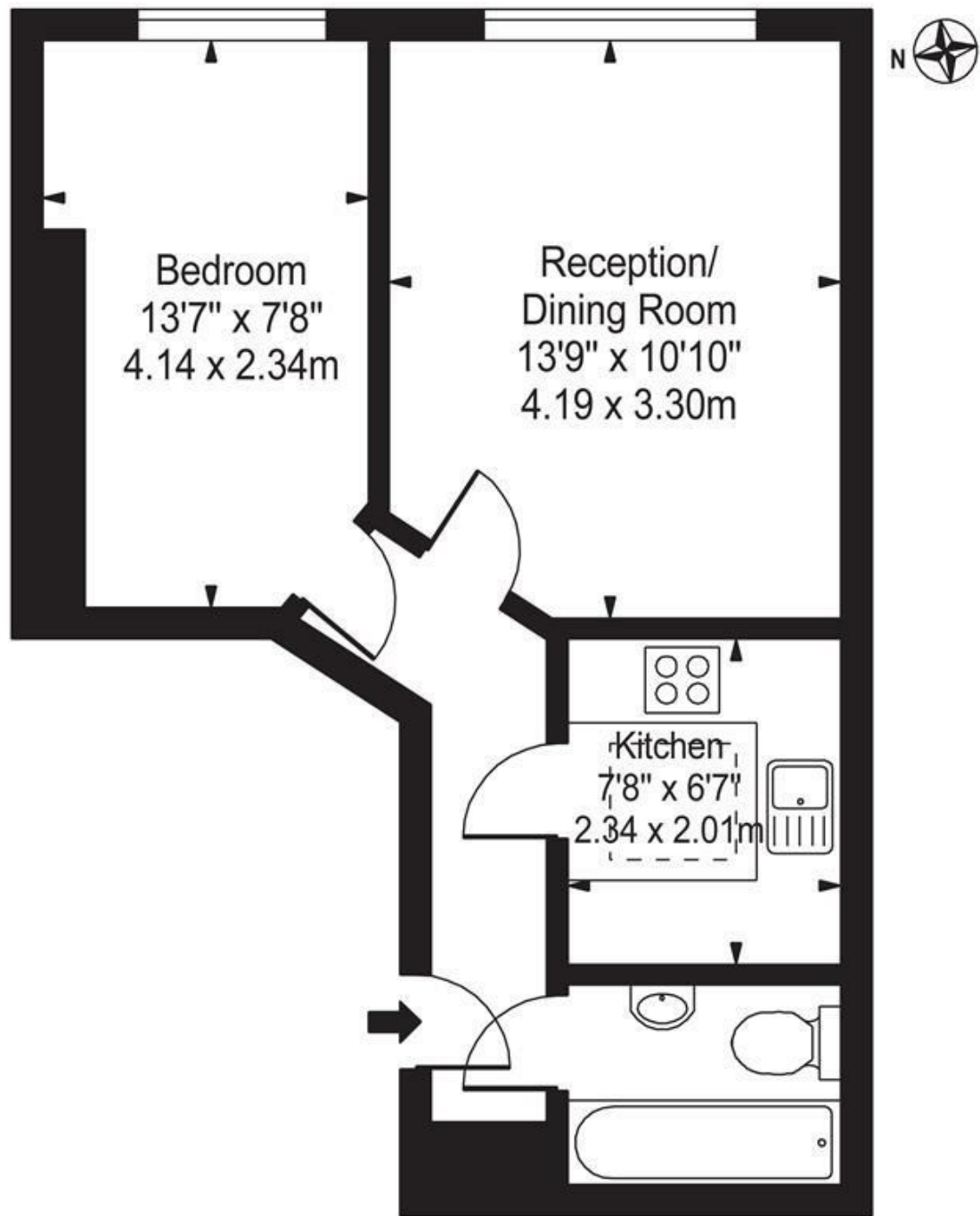
Third Floor
